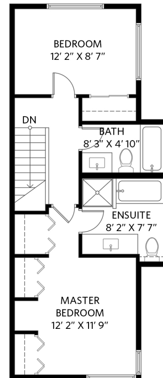
Upper Floor - 527 sq.ft. Ceiling height - 8' 0"
